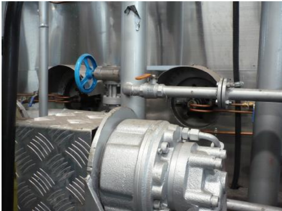
Burner – Diesel Type (2 units)
